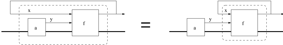
Figure 6: Interpreting axiom 2
