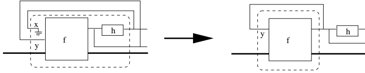
Figure 8: Interpreting equation 4
