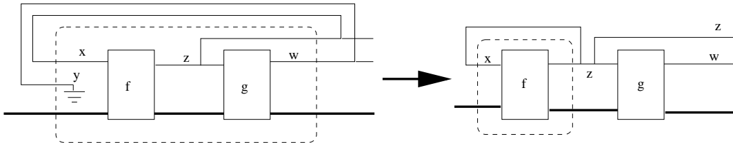
Figure 10: Interpreting equation 7
